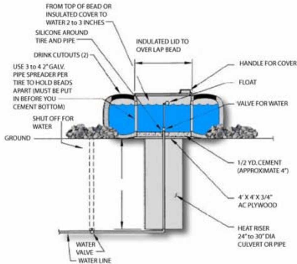
SIDE VIEW
