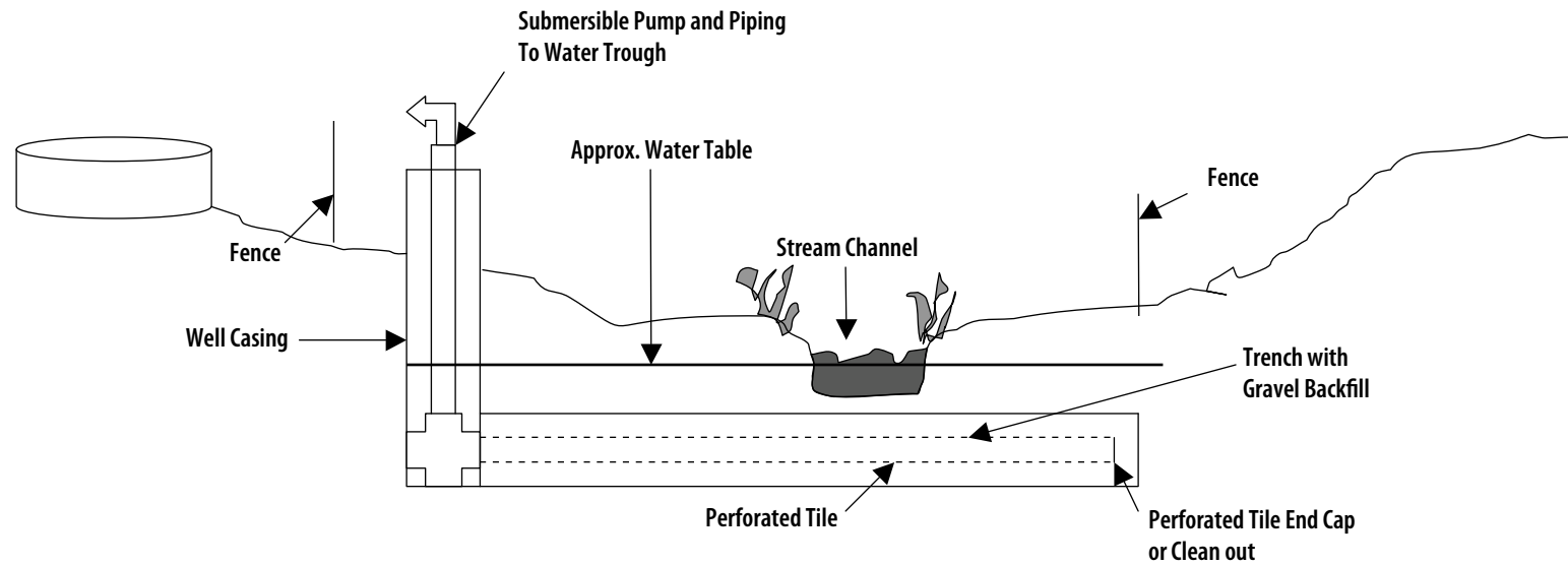
Horizontal Well Installation – Excavation Option
